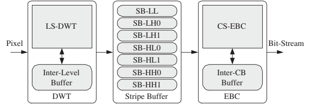
Fig. 4. Proposed JPEG 2000 architecture. No tile memory is required in the proposed architecture.
