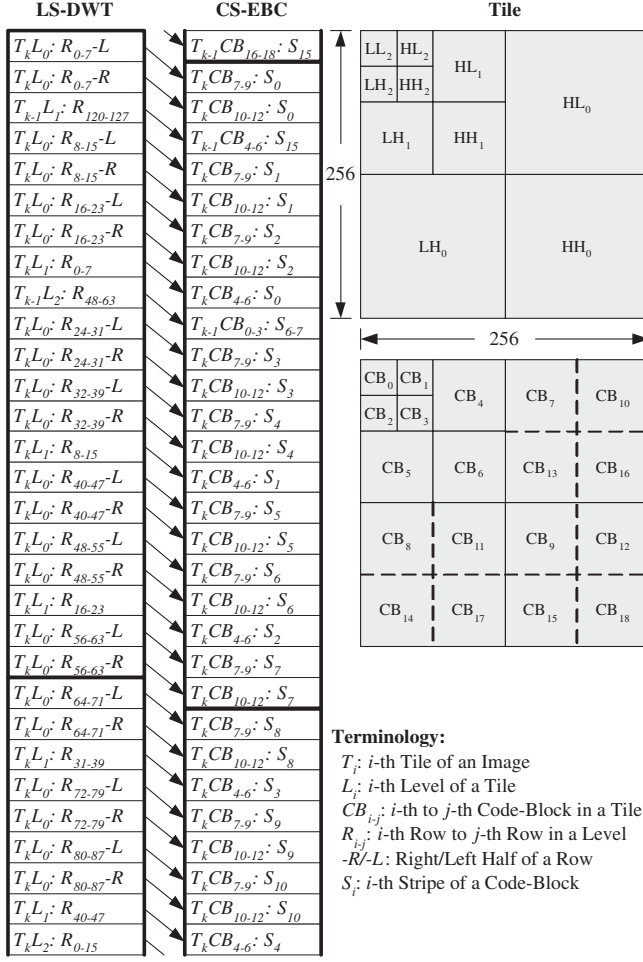
Fig. 5. Stripe pipeline scheme. The LS-DWT and CS-EBC are pipelined at stripe level, and therefore the buffer size is reduced to the same as the stripe size.
