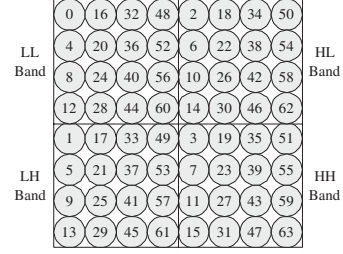
Fig. 3. Output order of DWT coefficients. The co-located DWT coefficients in all subbands are generated consequently.
