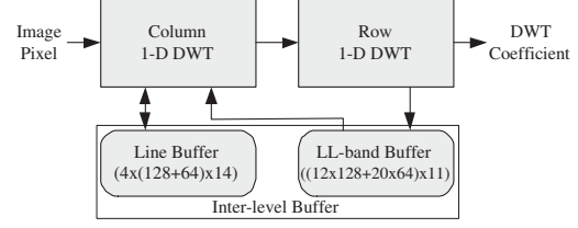
Fig. 6. Block diagram of the proposed LS-DWT. The LS-DWT can transform 3 levels in parallel.
