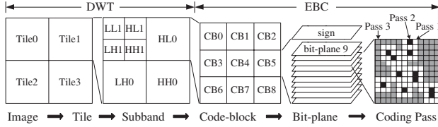
Fig. 1. JPEG 2000 coding system. It adopts the DWT as the transform algorithm and the EBCOT as the entropy coding algorithm.
