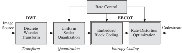
Fig. 1. JPEG 2000 coding system. It adopts the DWT as the transform algorithm and the EBCOT as the entropy coding algorithm.
